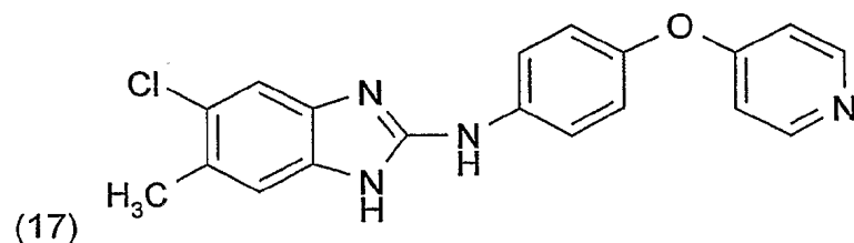
(5-Chlor-6-methyl-1H-benzimidazol-2-yl)-[4-(pyridin-4-yloxy)-phenyl]-amin
